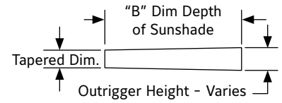
Tapered Outrigger
