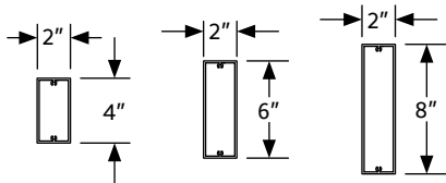
Tube Fascia
