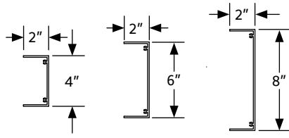
Channel Fascia
