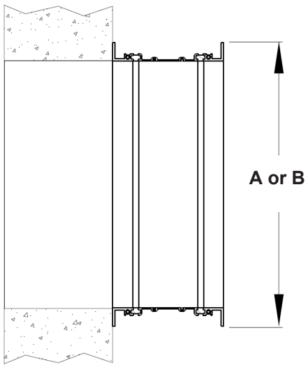
Thermal Broke Frame On Wall Opening A x B dimensions are to O.D. of damper frame
