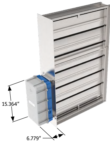
Enclosure mounted external on extended shaft
