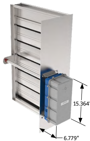
Enclosure mounted external on jackshaft
