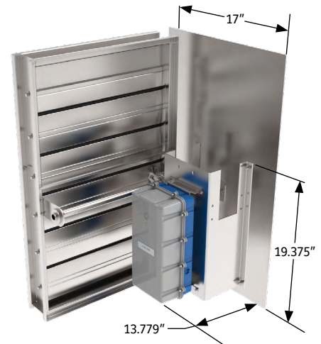
Enclosure mounted internal on jackshaft
